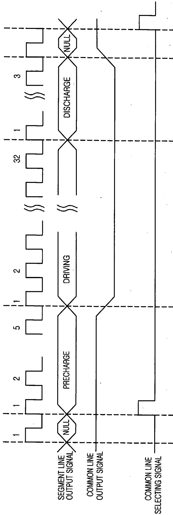
FIG. 4 (PRIOR ART)
